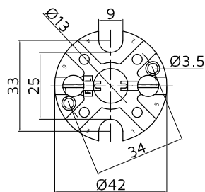
TBB500-AD
