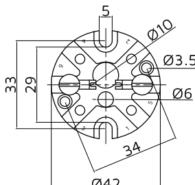
TBB670-AD
