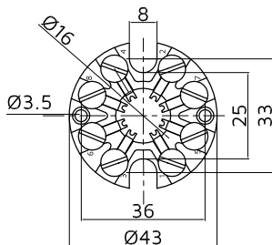
TBB850-AD
