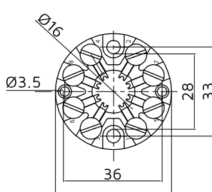
TBB800-AD
